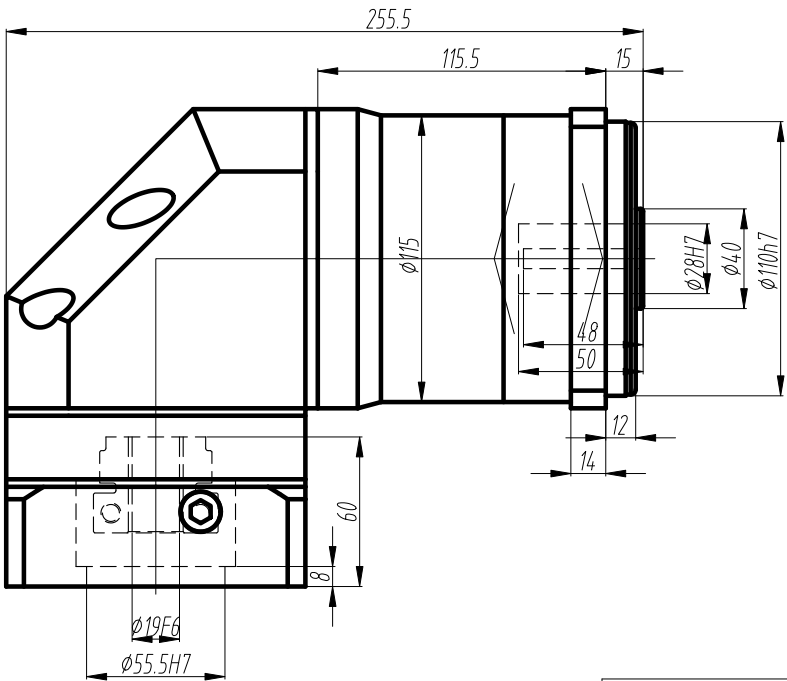
标准轴 Standard output shaft
